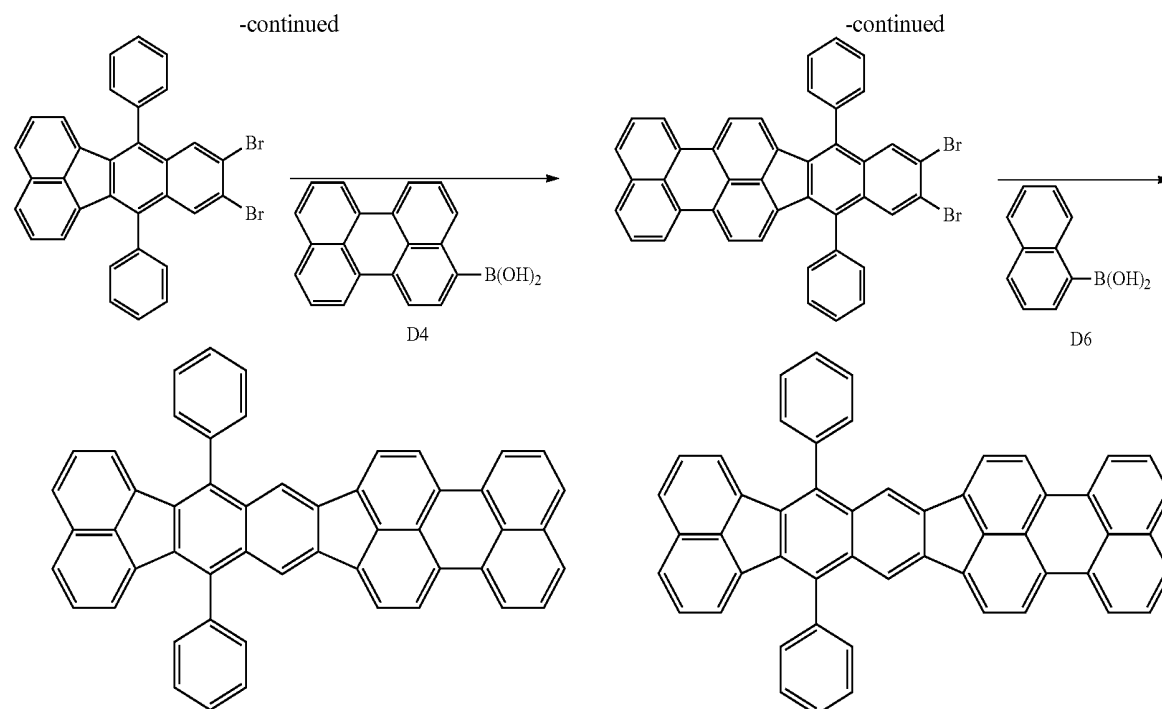
Synthesis route 2
