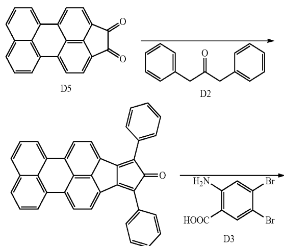
Synthesis route 2
