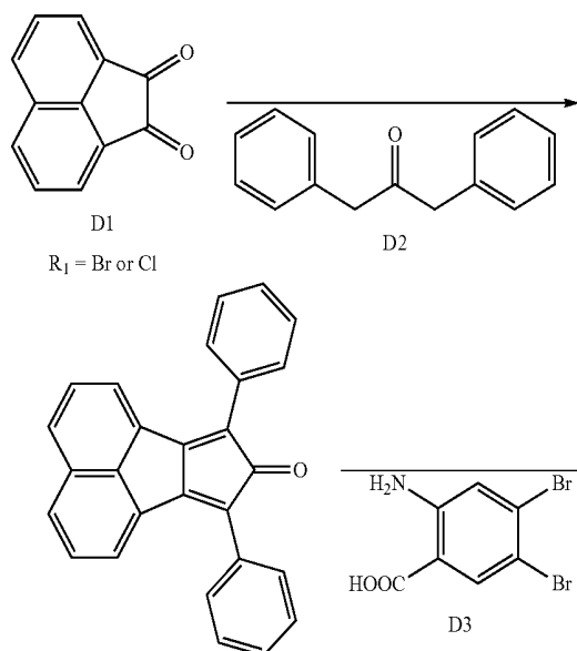
Synthesis route 1
